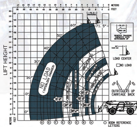
STANDARD FORK FRAME REACH
